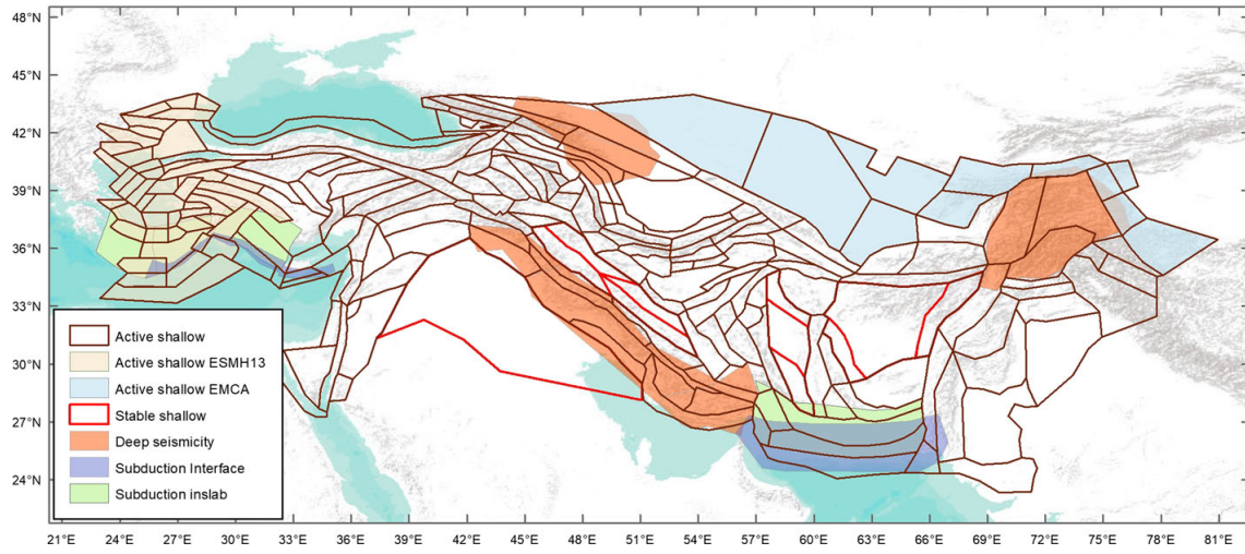
Figure 1 – EMME area source model. From Danciu et al. (2017)
