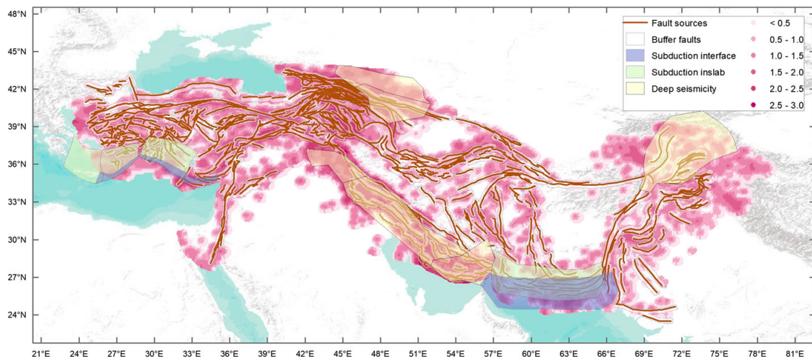
Figure 2 – EMME fault source and background seismicity model. From Danciu et al. (2017)
